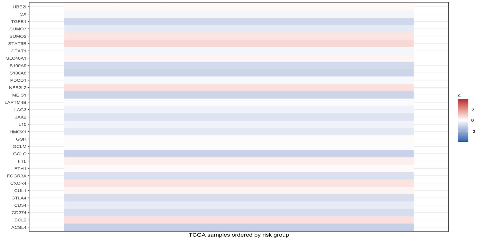
Key gene expression in high- vs low-risk groups
