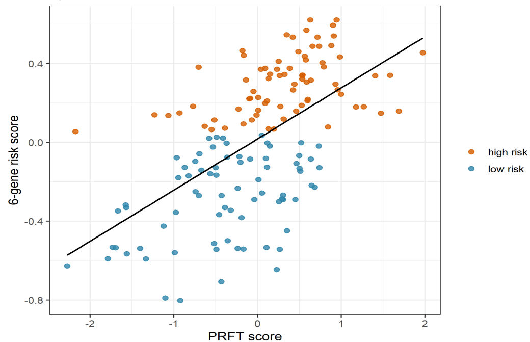
Risk score vs PRFT score Spearman rho = 0.593, P = 1.11e-15
